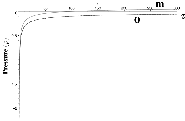
Fig. 1. Evolution of the pressure with the expansion of the BI Universe when it is filled with perfect fluid and dark energy obeying ordinary and modified quintessence given by (3.8) and (3.9), respectively. Here the letters “o” and “m” stand for ordinary and modified, respectively.
