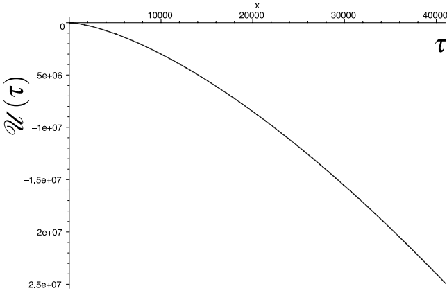
Fig. 2. View of the potential when the BI Universe is filled with a binary mixture of perfect fluid and a quintessence given by (3.8).
