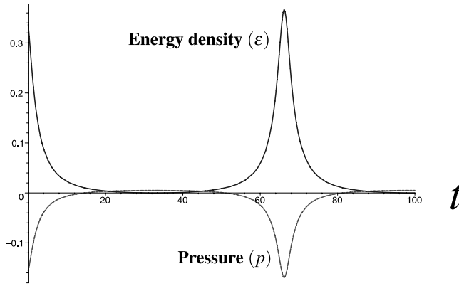
Fig. 7. View of energy density and pressure when BI Universe experiences oscillation as in Fig. 6.
